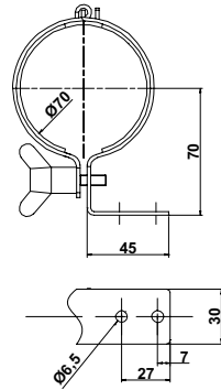
190-015-995 Strap Bracket – Short-L
