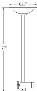
Ceiling Mount: • 8-9 ft. = 25" • 10 ft. = 40"
