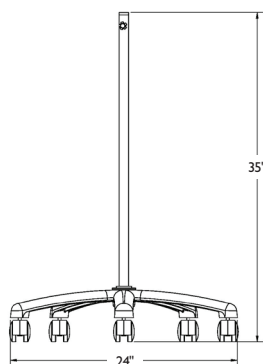
Floor Stand
